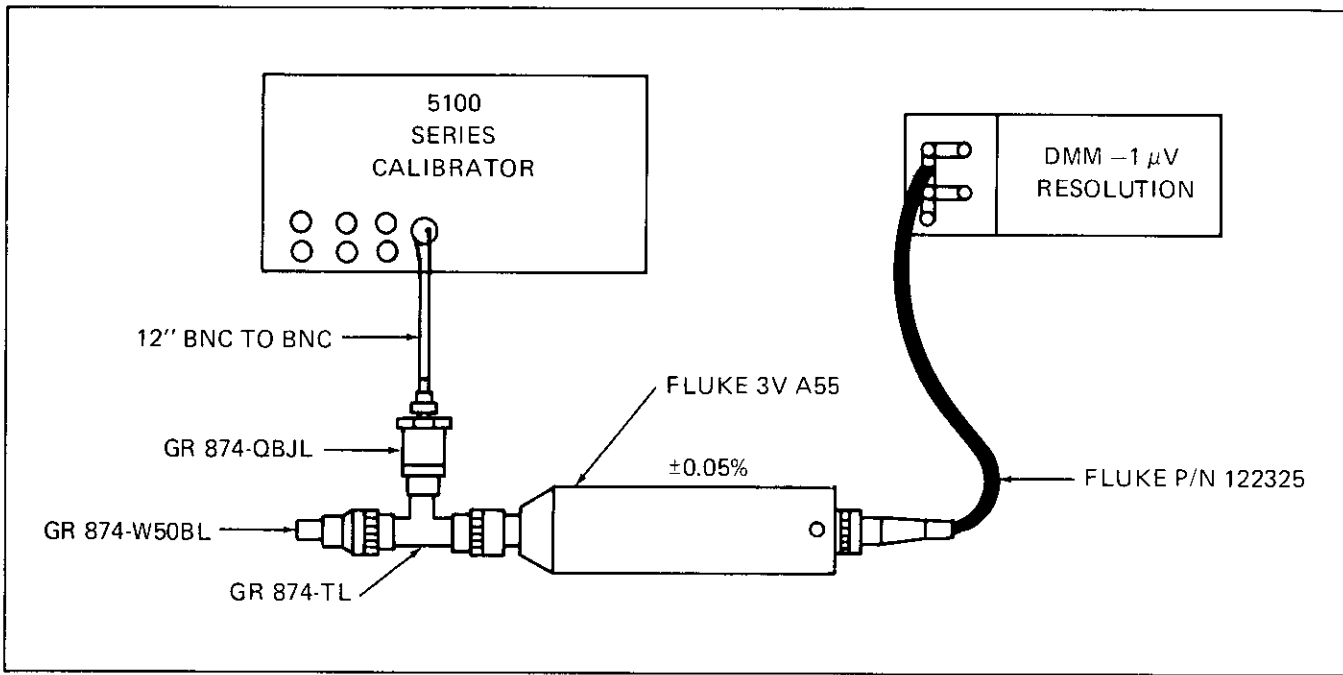
Figure 603-3. Wideband Low Frequency Flatness Tests
