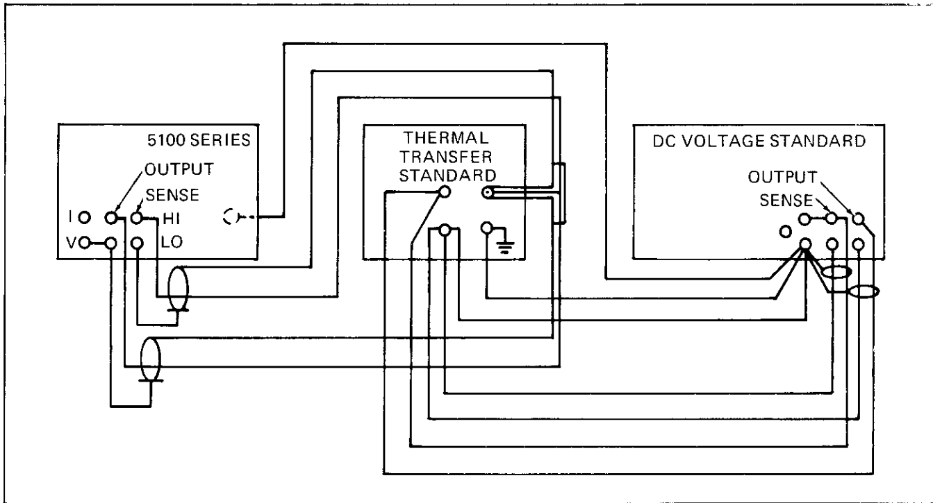
Figure 4-7. AC Voltage Tests
