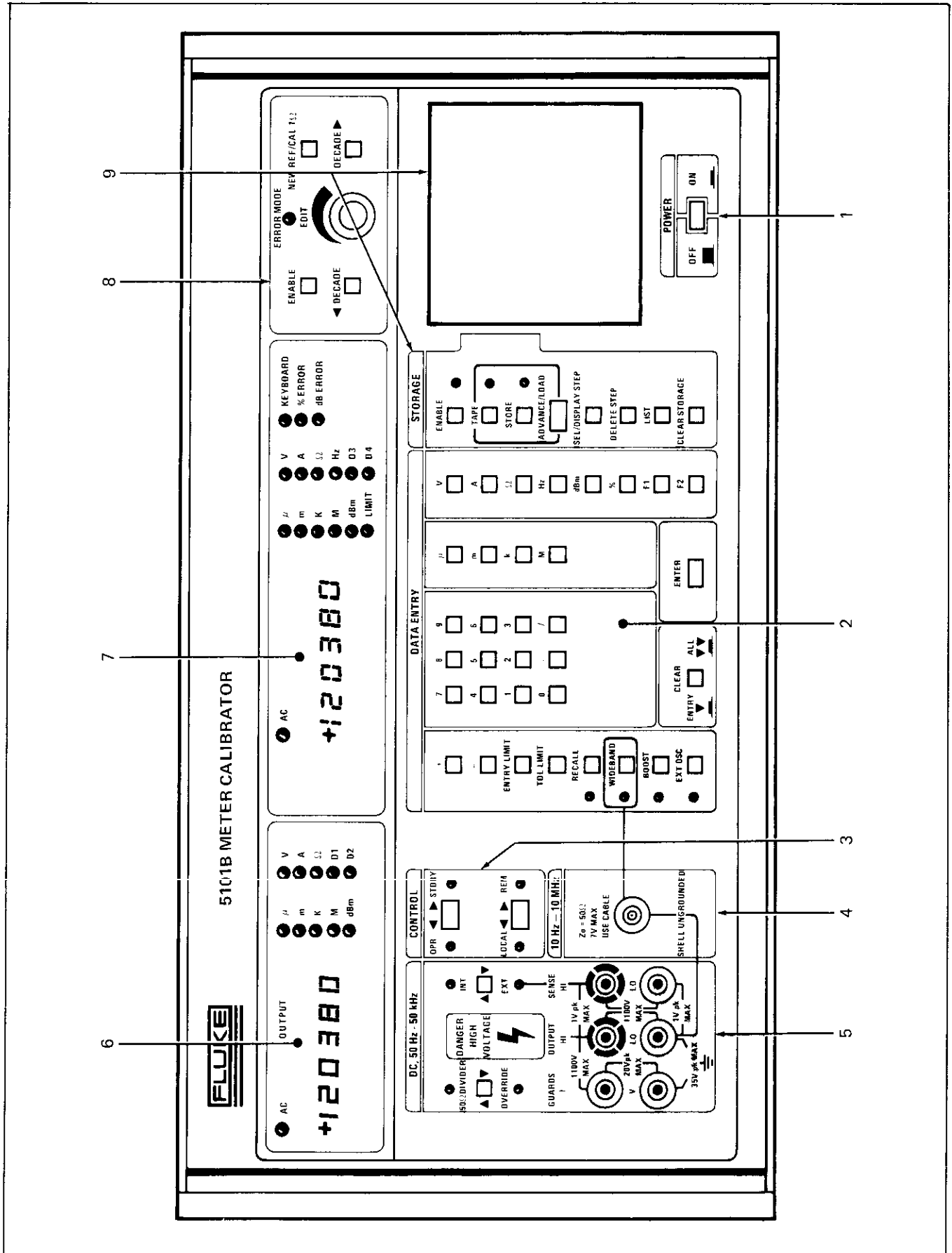
Figure 2-1. Front Panel
