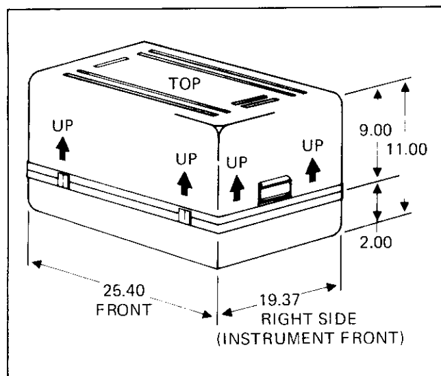
Figure 600-1. Transit Case
