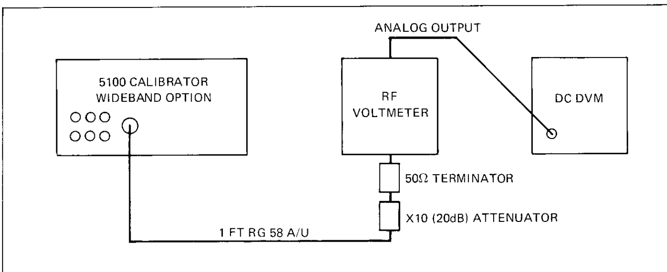
Figure 603-6. Wideband Medium and High Frequency Flatness Tests
