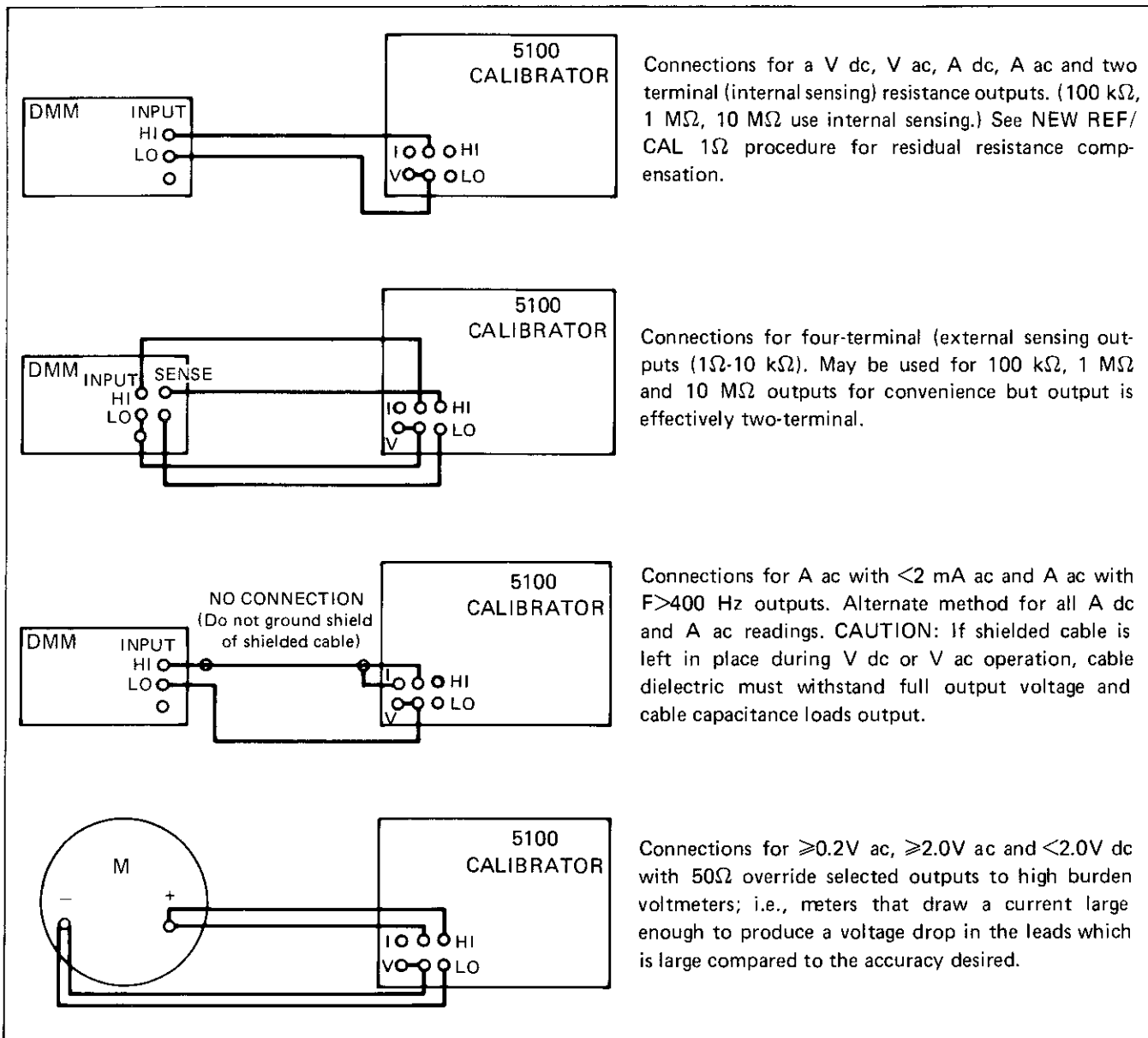
Figure 2-12. Meter Connections
