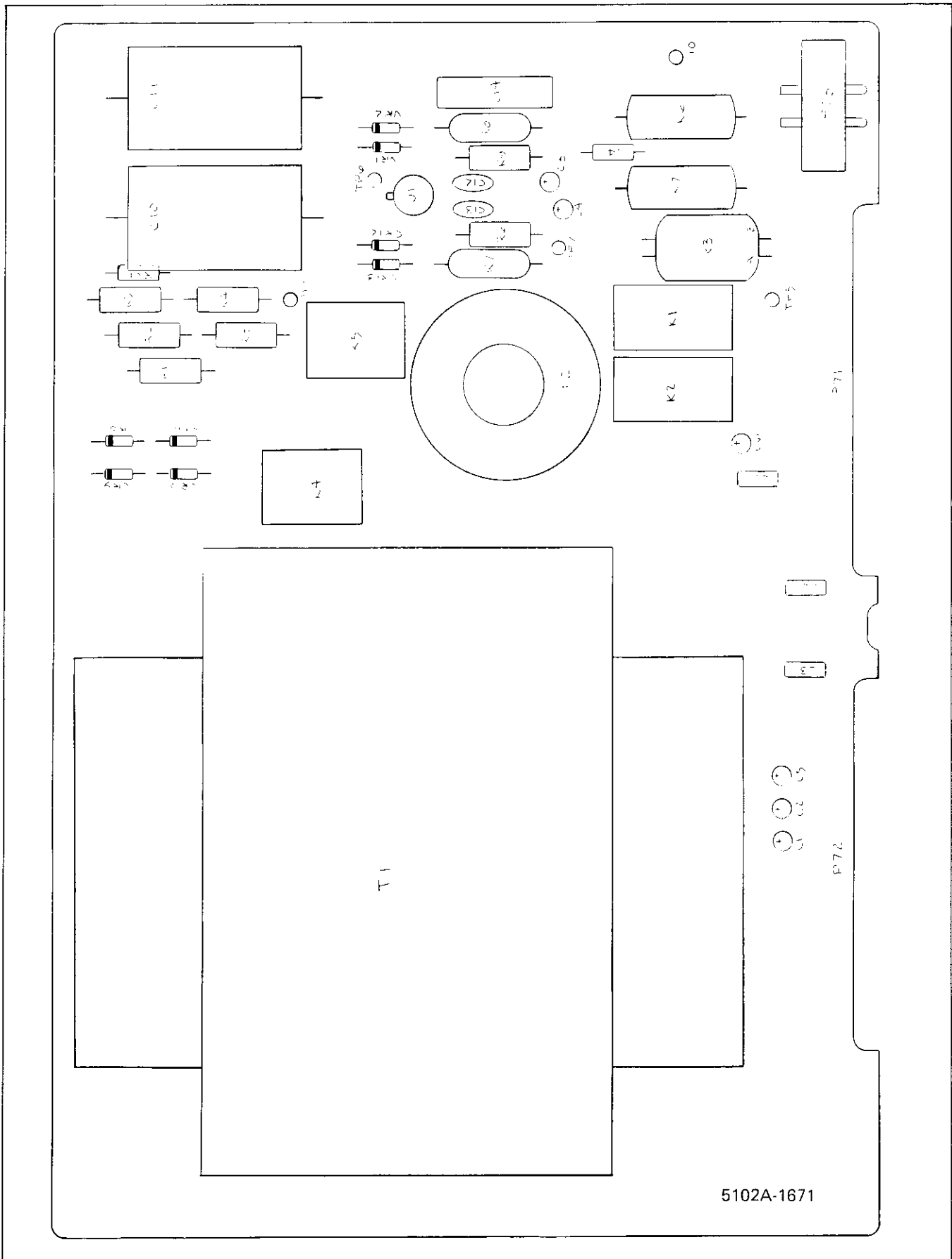
Figure 5-18. A16 Extended High Voltage PCB Assembly, Environmental Case
