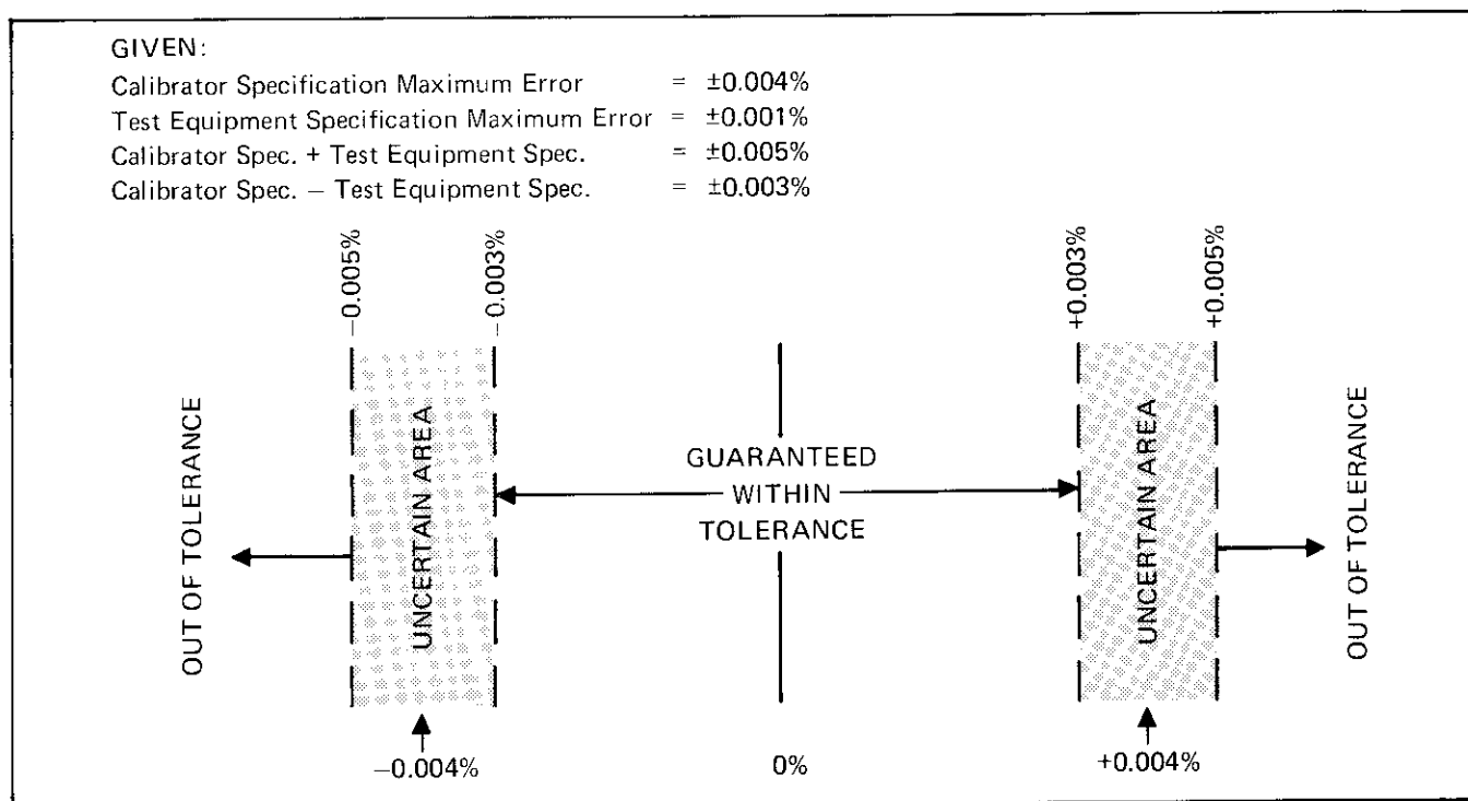
Figure 4-2. Accuracy Uncertainties
